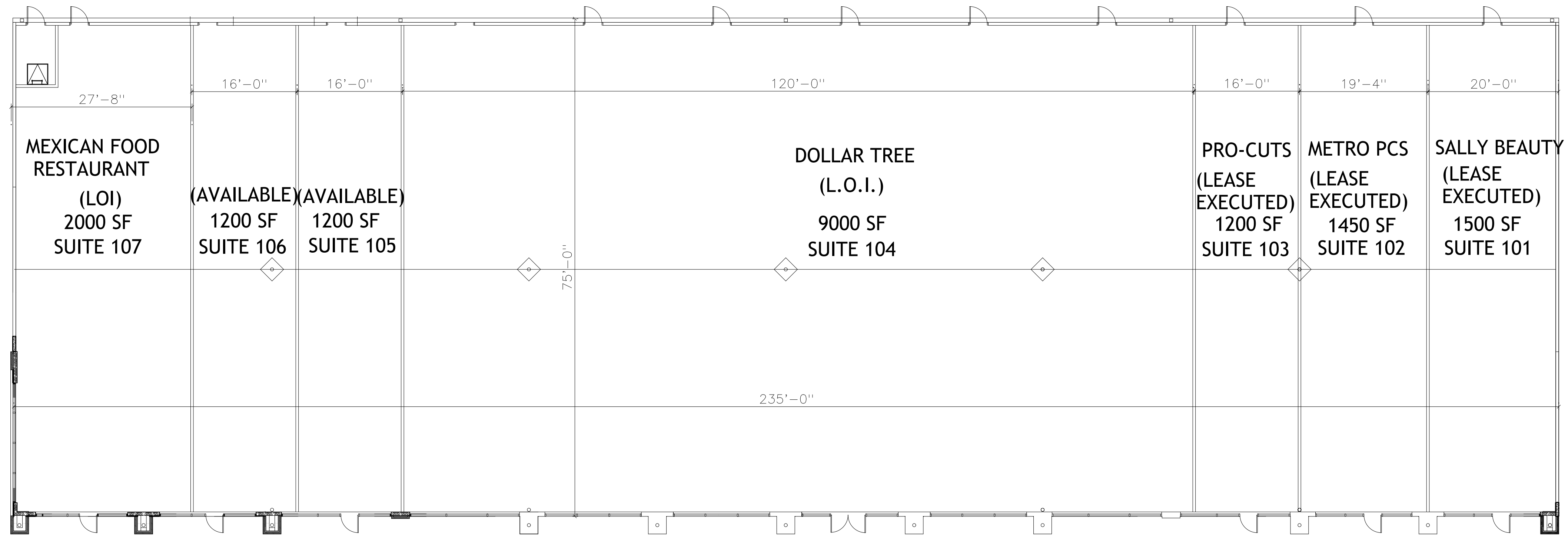
FLOOR PLAN
